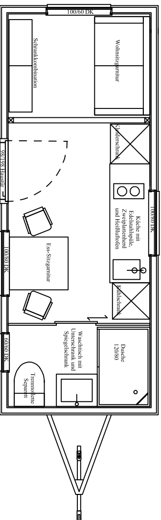
Tiny House 6,20m x 2,49m
