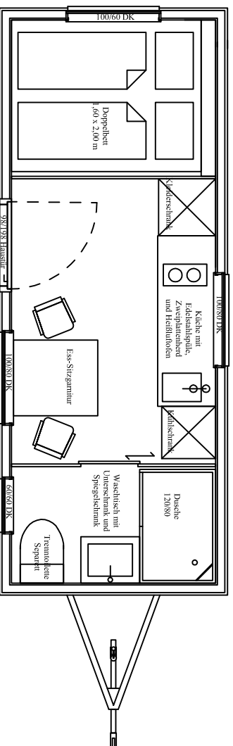
Tiny House 6,20m x 2,49m
